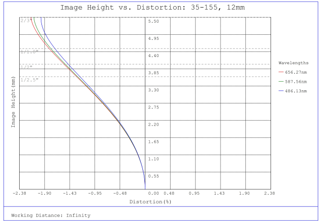
#35-155, 12mm, f/1.8 Cr Series Fixed Focal Length Lens, Distortion Plot
