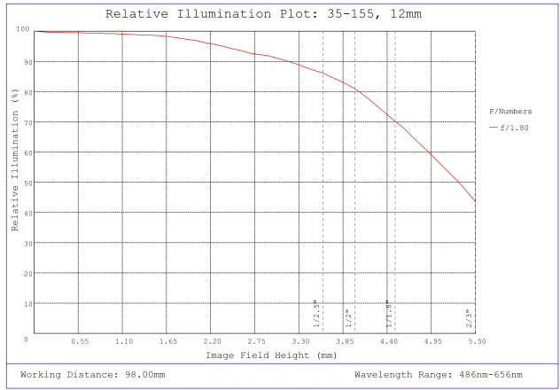
#35-155, 12mm, f/1.8 Cr Series Fixed Focal Length Lens, Relative Illumination Plot
