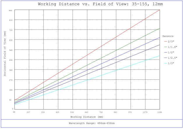
#35-155, 12mm, f/1.8 Cr Series Fixed Focal Length Lens, Working Distance versus Field of View Plot
