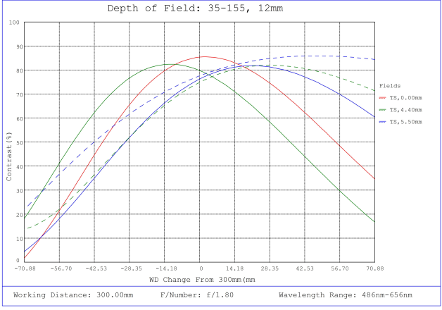
#35-155, 12mm, f/1.8 Cr Series Fixed Focal Length Lens, Depth of Field Plot, 300mm Working Distance, f1.8
