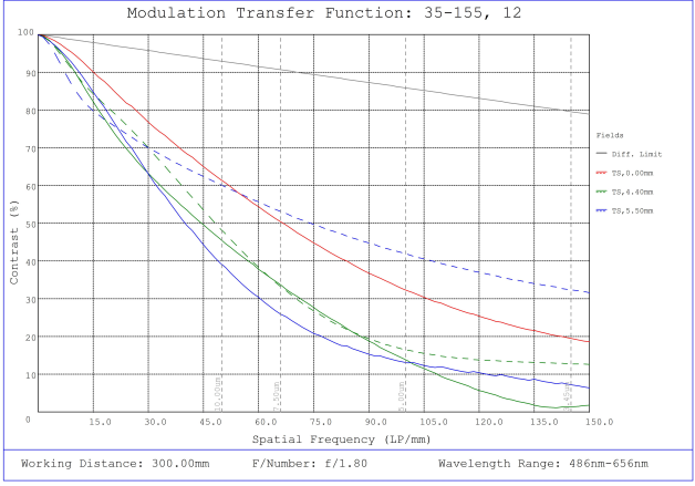
#35-155, 12mm, f/1.8 Cr Series Fixed Focal Length Lens, Modulated Transfer Function (MTF) Plot, 300mm Working Distance, f1.8
