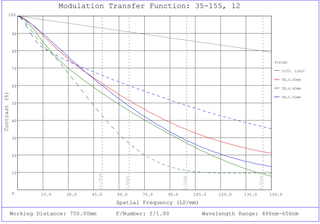
#35-155, 12mm, f/1.8 Cr Series Fixed Focal Length Lens, Modulated Transfer Function (MTF) Plot, 750mm Working Distance, f1.8
