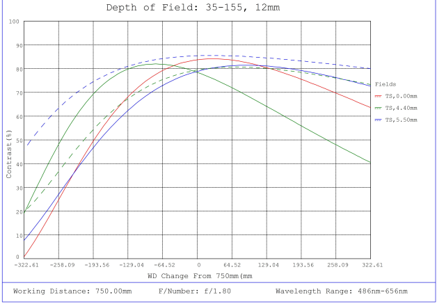
#35-155, 12mm, f/1.8 Cr Series Fixed Focal Length Lens, Depth of Field Plot, 750mm Working Distance, f1.8
