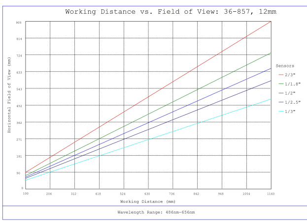
#36-857, 12mm f/5.6, 1000mm-∞ Primary WD, HRr Series Fixed Focal Length Lens, Working Distance versus Field of View Plot
