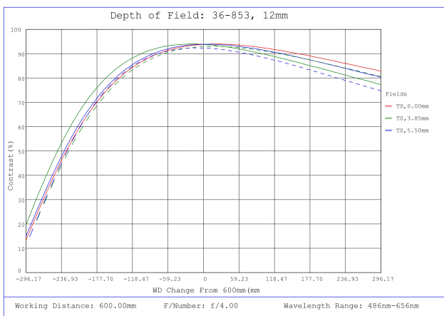
#36-853, 12mm f/4, 400-2000mm Primary WD, HRr Series Fixed Focal Length Lens, Depth of Field Plot, 600mm Working Distance, f4
