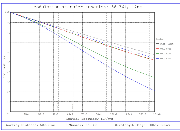
#36-761, 12mm f/4, 400-2000mm Primary WD, HRI Series Fixed Focal Length Lens, Modulated Transfer Function (MTF) Plot, 500mm Working Distance, f4
