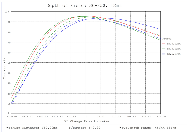
#36-850, 12mm f/2.8, 400-2000mm Primary WD, HRr Series Fixed Focal Length Lens, Depth of Field Plot, 650mm Working Distance, f2.8
