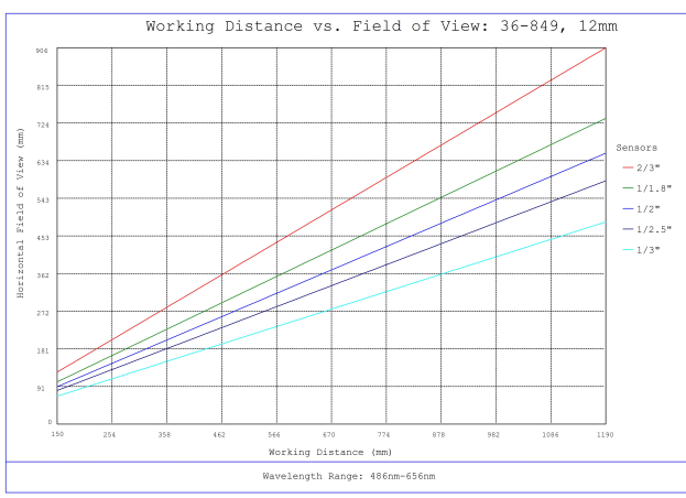
#36-849, 12mm f/2.8, 150-500mm Primary WD, HRr Series Fixed Focal Length Lens, Working Distance versus Field of View Plot
