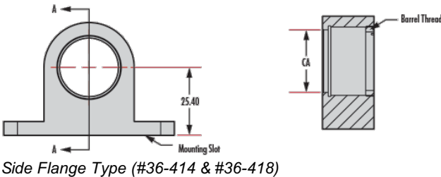
Side Flange Type (#36-414 & #36-418)
