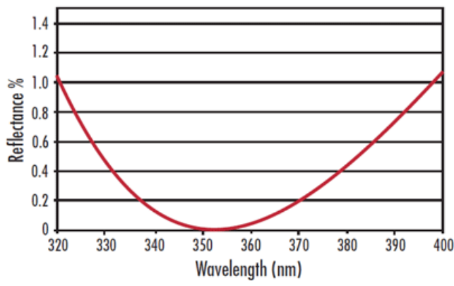
355nm V-Coat R_{(abs)} < 0.25\% @ 355nm
