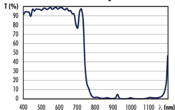
IR Cutoff Filter Coating Performance
