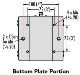
Bottom Plate Portion
