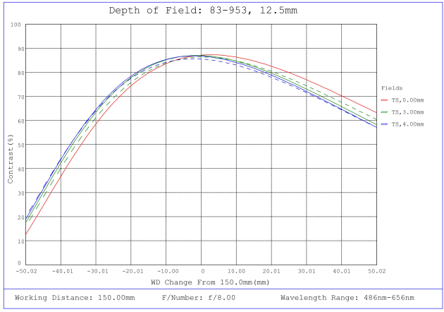
#83-953, 12.5mm FL f/8, Blue Series M12 Lens, Depth of Field Plot, 150mm Working Distance, f8
