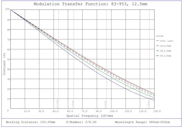
#83-953, 12.5mm FL f/8, Blue Series M12 Lens, Modulated Transfer Function (MTF) Plot, 150mm Working Distance, f8
