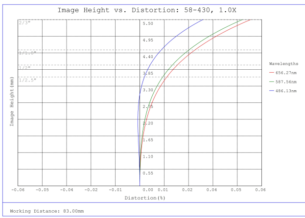
#58-430, 1.0X SilverTL™ Telecentric Lens, Distortion Plot
