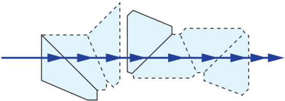
Schmidt-Pechan Prism Tunnel Diagram
