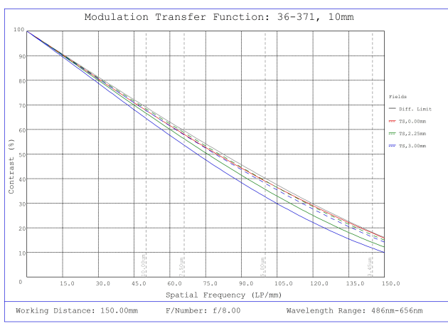
#36-371, 10mm FL f/8, Rugged Blue Series M12 Lens, Modulated Transfer Function (MTF) Plot, 150mm Working Distance, f8
