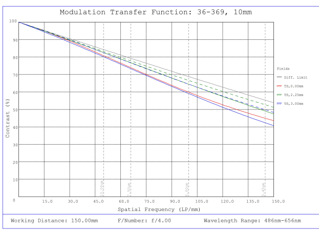
#36-369, 10mm FL f/4, Rugged Blue Series M12 Lens, Modulated Transfer Function (MTF) Plot, 150mm Working Distance, f4
