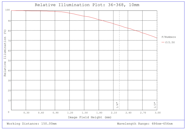
#36-368, 10mm FL f/2.5, Rugged Blue Series M12 Lens, Relative Illumination Plot
