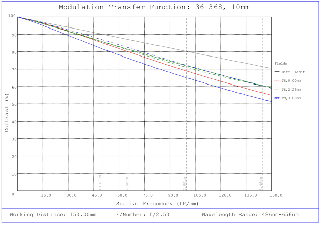
#36-368, 10mm FL f/2.5, Rugged Blue Series M12 Lens, Modulated Transfer Function (MTF) Plot, 150mm Working Distance, f2.5
