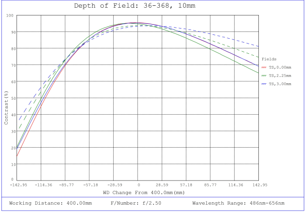
#36-368, 10mm FL f/2.5, Rugged Blue Series M12 Lens, Depth of Field Plot, 400mm Working Distance, f2.5
