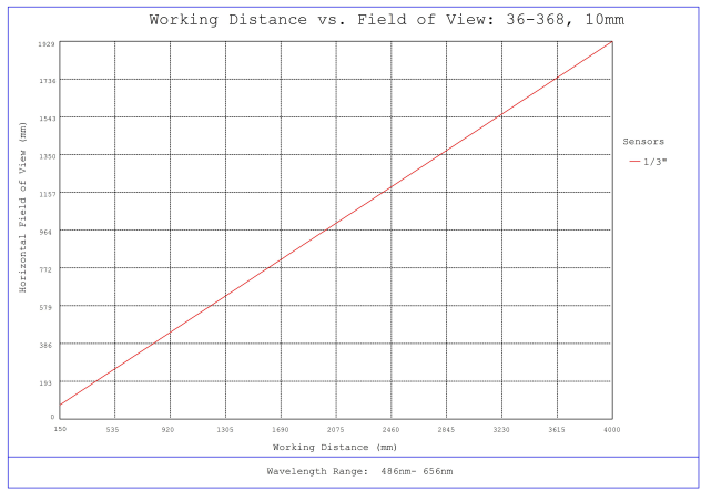
#36-368, 10mm FL f/2.5, Rugged Blue Series M12 Lens, Working Distance versus Field of View Plot
