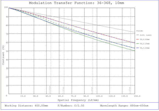
#36-368, 10mm FL f/2.5, Rugged Blue Series M12 Lens, Modulated Transfer Function (MTF) Plot, 400mm Working Distance, f2.5
