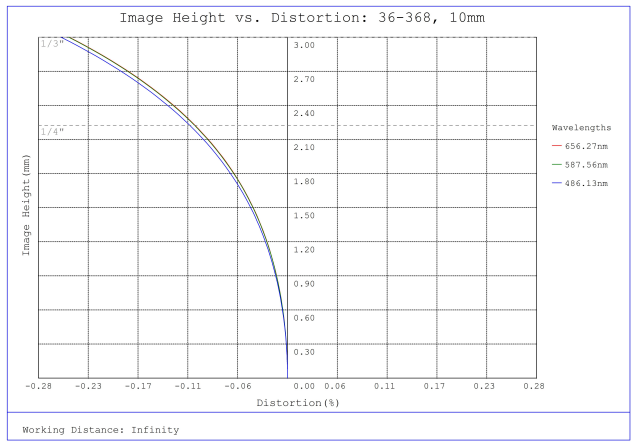
#36-368, 10mm FL f/2.5, Rugged Blue Series M12 Lens, Distortion Plot
