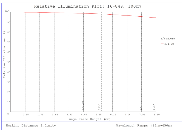
#16-849, 100mm, f/4 Athermal Lens, Relative Illumination Plot
