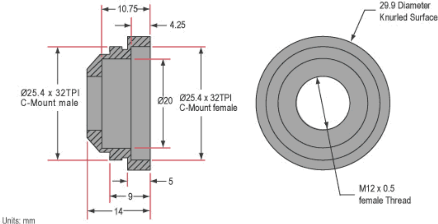
C-Mount Adapter (#53-675)
