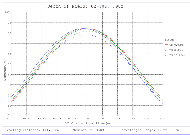
#62-902, 0.9X, 28.7mm F-Mount PlatinumTL™ Telecentric Lens, Depth of Field Plot, 111mm Working Distance, f10
