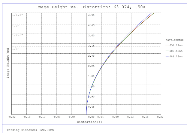
#63-074, 0.50X SilverTL™ Telecentric Lens, Distortion Plot
