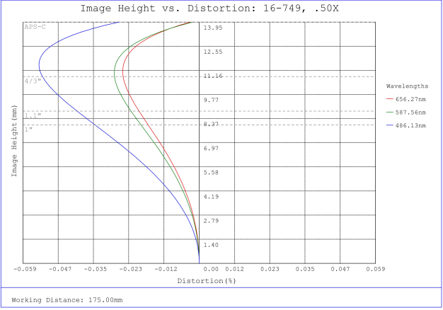
#16-749, 0.5X, 28.7mm TFL-Mount PlatinumTL™ Telecentric Lens, Distortion Plot
