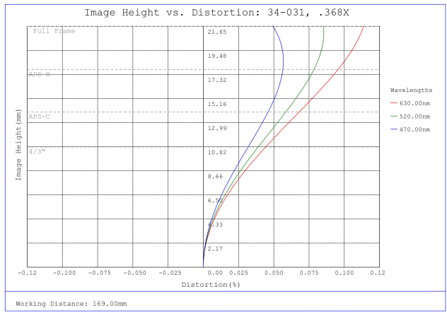
#34-031, 0.368X, 35mm F-Mount TitanTL® Telecentric Lens, Distortion Plot
