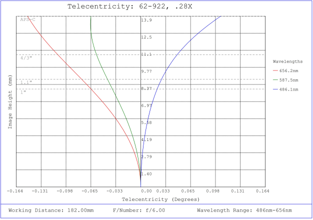
#62-922, 0.28X, 28.7mm F-Mount PlatinumTL™ Telecentric Lens, Telecentricity Plot
