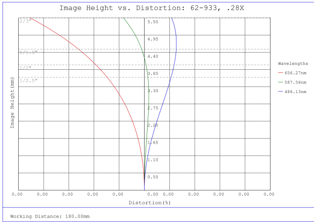
#62-933, 0.28X, 2/3" C-Mount PlatinumTL™ Telecentric Lens, Distortion Plot
