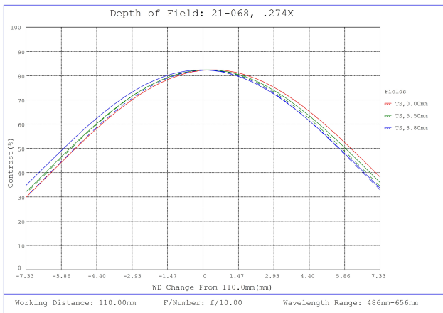
#21-068, 0.274X CobaltTL Telecentric Lens, Depth of Field Plot, 110mm Working Distance, f10
