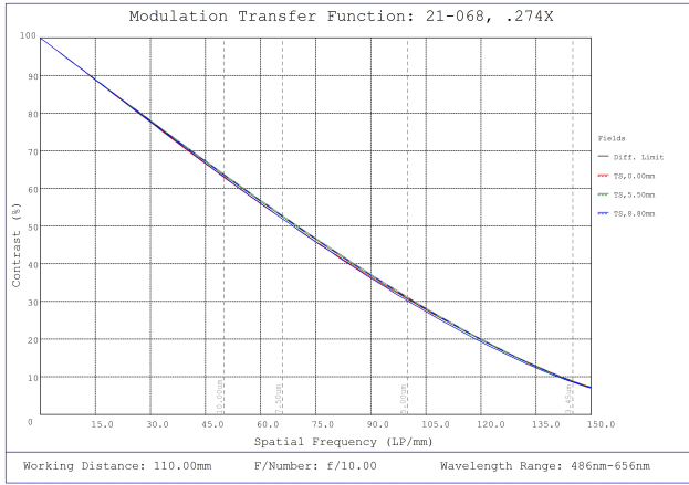
#21-068, 0.274X CobaltTL Telecentric Lens, Modulated Transfer Function (MTF) Plot, 110mm Working Distance, f10
