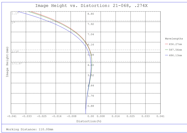
#21-068, 0.274X CobaltTL Telecentric Lens, Distortion Plot
