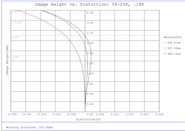
#58-258, 0.18X 1/2" GoldTL™ Telecentric Lens, Distortion Plot
