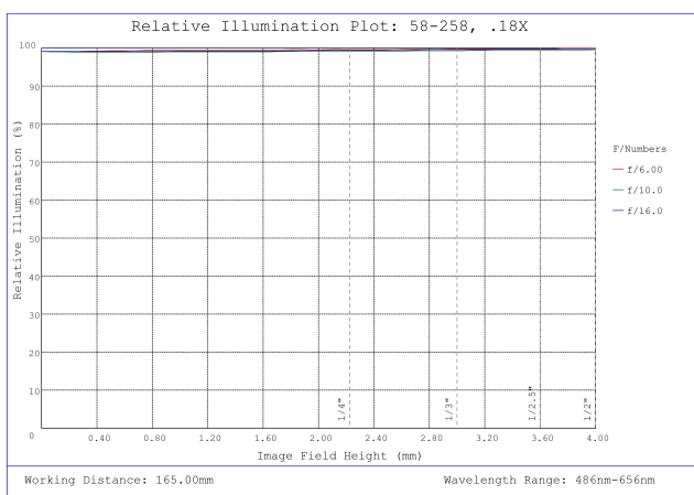
#58-258, 0.18X 1/2" GoldTL™ Telecentric Lens, Relative Illumination Plot
