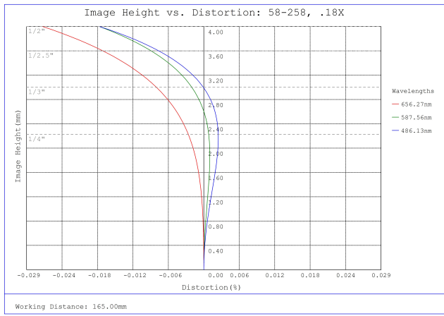
#58-258, 0.18X 1/2" GoldTL™ Telecentric Lens, Distortion Plot
