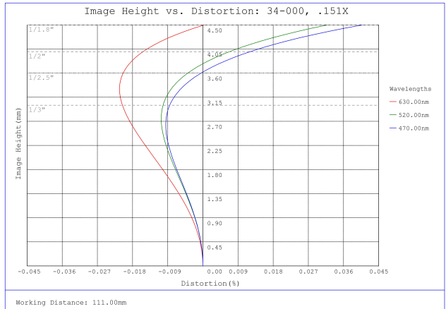
#34-000, 0.151X, 1/1.8" C-Mount TitanTL® Telecentric Lens, Distortion Plot
