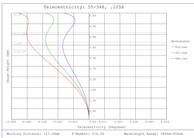
#55-348, 0.125X, 2/3" GoldTL™ Telecentric Lens, Telecentricity Plot
