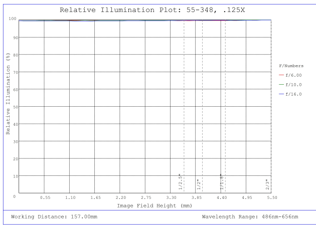
#55-348, 0.125X, 2/3" GoldTL™ Telecentric Lens, Relative Illumination Plot
