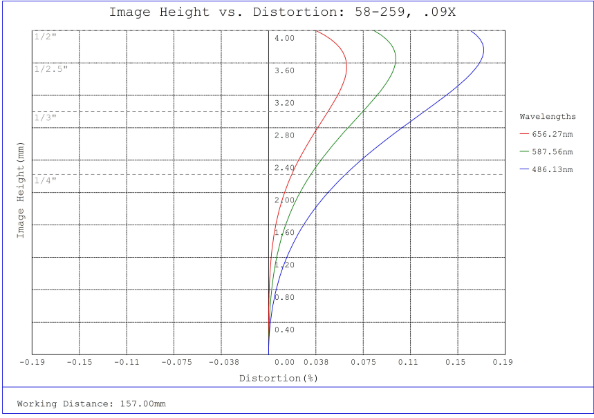
#58-259, 0.09X ½" GoldTL™ Telecentric Lens, Distortion Plot
