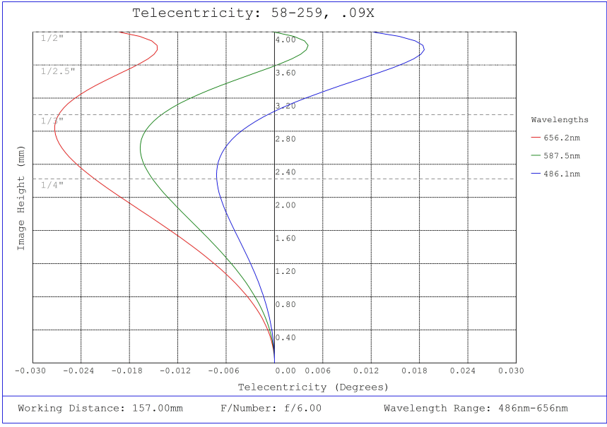
#58-259, 0.09X ½" GoldTL™ Telecentric Lens, Telecentricity Plot
