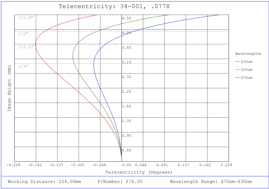
#34-001, 0.077X, 1/1.8" C-Mount TitanTL® Telecentric Lens, Telecentricity Plot
