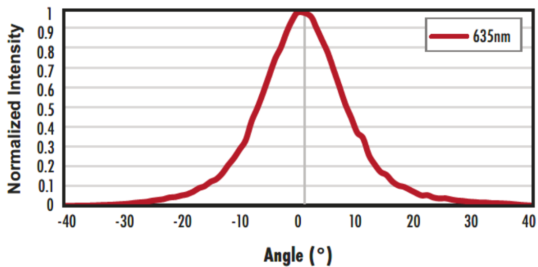
Relative Intensity vs. Angle Light Diffusing Film
