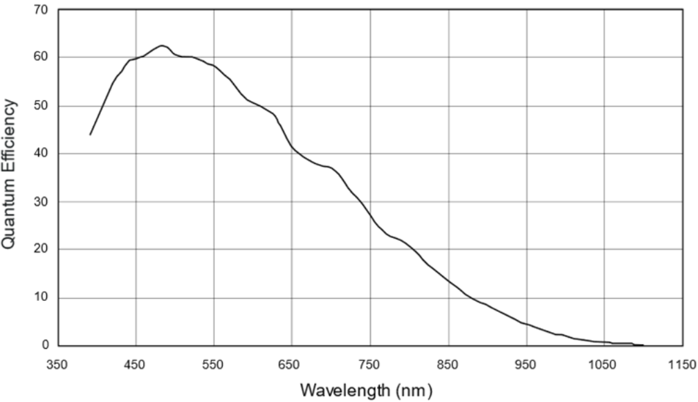
MT9P031 Sensor QE Curve
