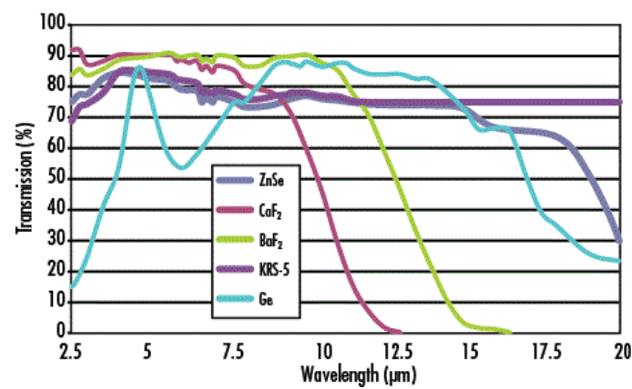
Typical Max Transmission for Linear Polarized Light
