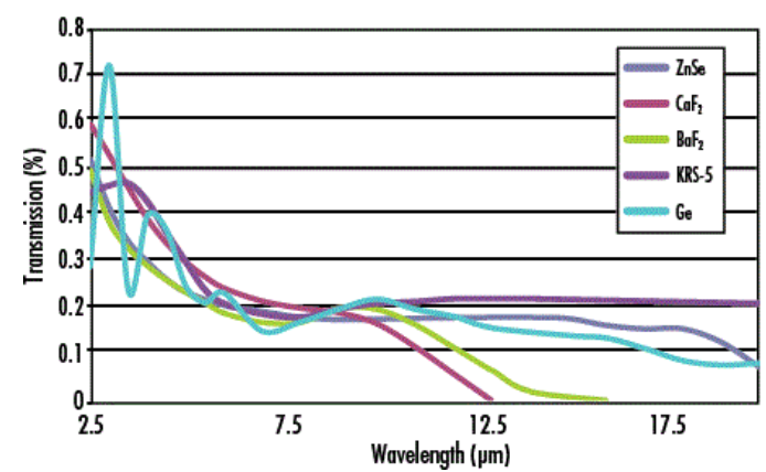
Typical Min Transmission for Linear Polarized Light
