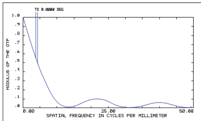
Typical Performance 25mm diameter, 60mm focal length PCX Lens (Monochromatic Illumination)
