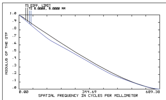
Typical Performance, #47-443 GRADIUM® Lens (Monochromatic Illumination)
