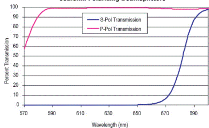
632.8nm Polarizing Beamsplitters
