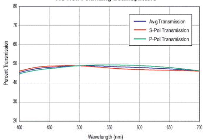
VIS Non-Polarizing Beamsplitters
