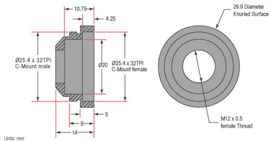
C-Mount Adapter (#53-675)
