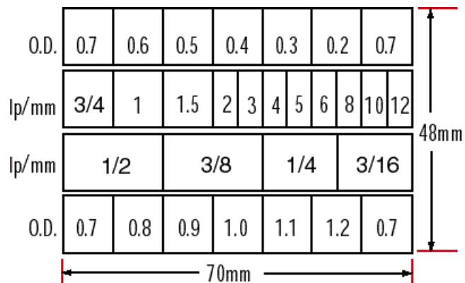
Reflected Target #54-804
