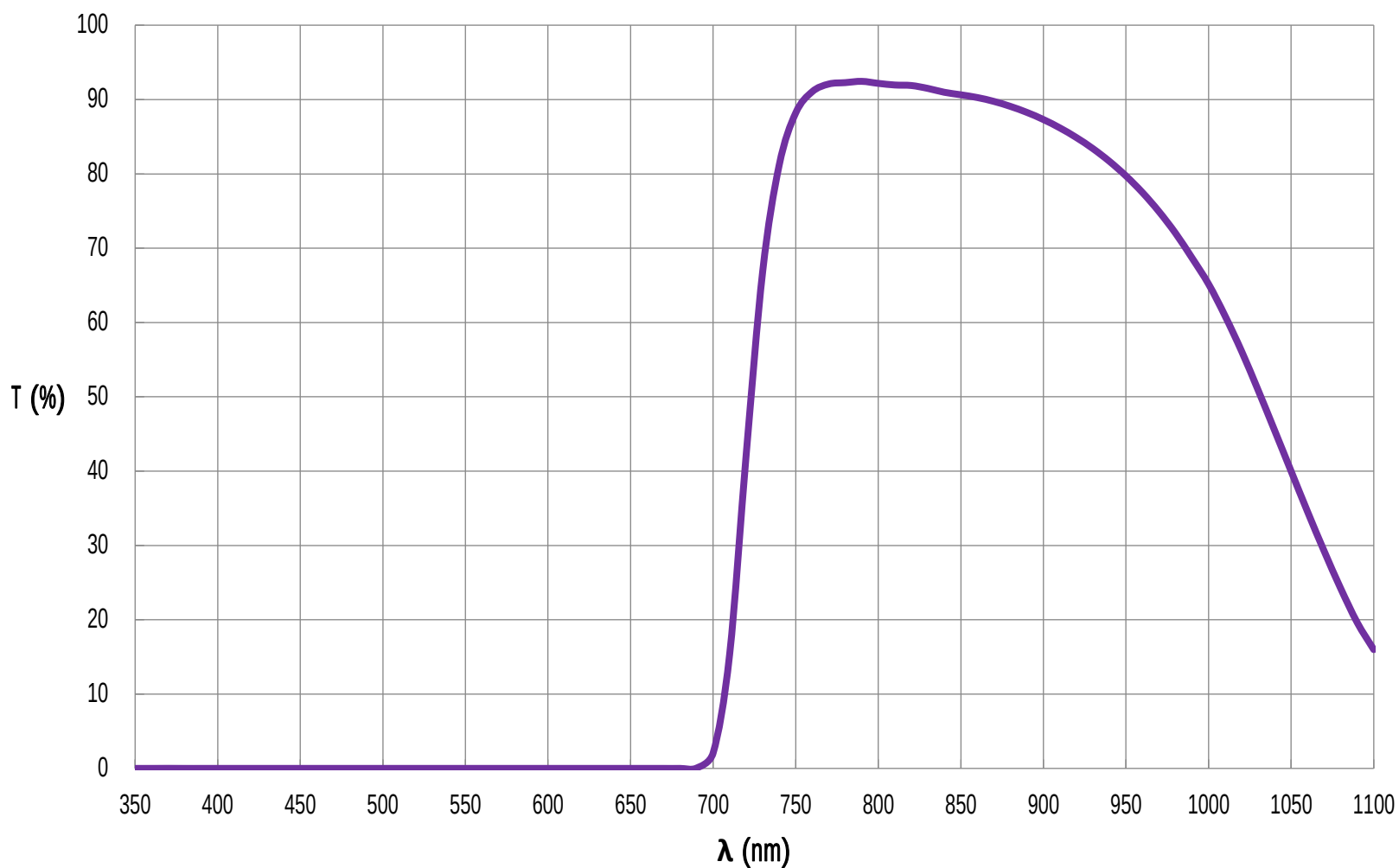
Near-IR Machine Vision Bandpass Filter, 800nm FOR REFERENCE ONLY
