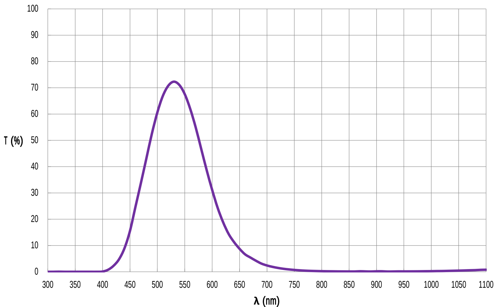
Photopic Response Filter, 530nm FOR REFERENCE ONLY
