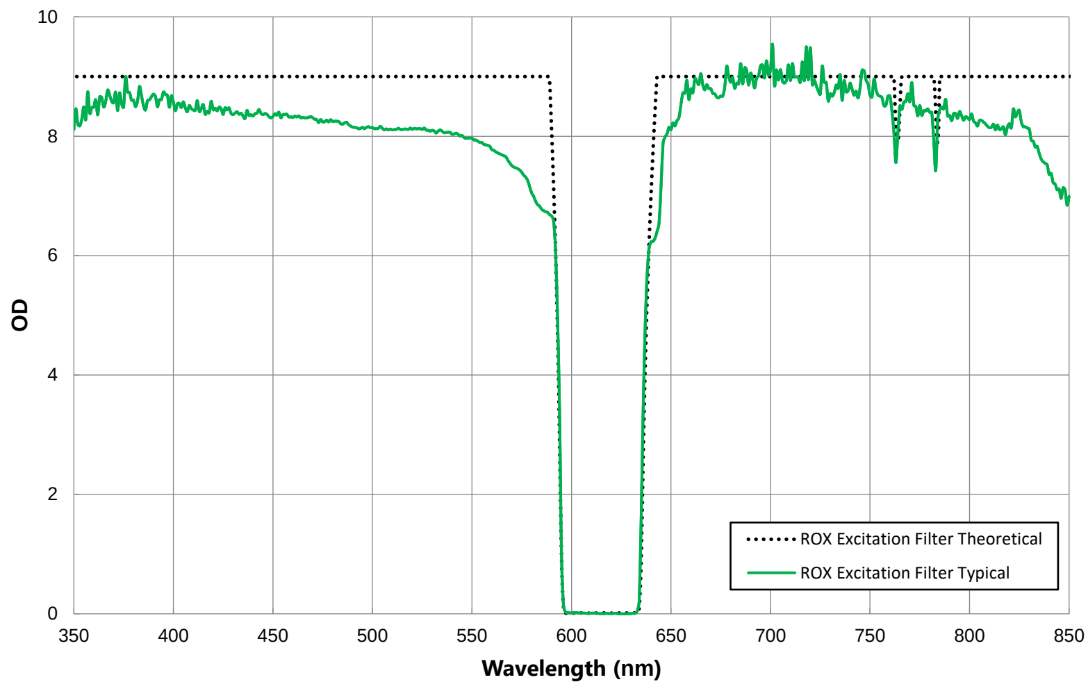
615nm CWL, OD8 High Blocking Bandpass Filter FOR REFERENCE ONLY
