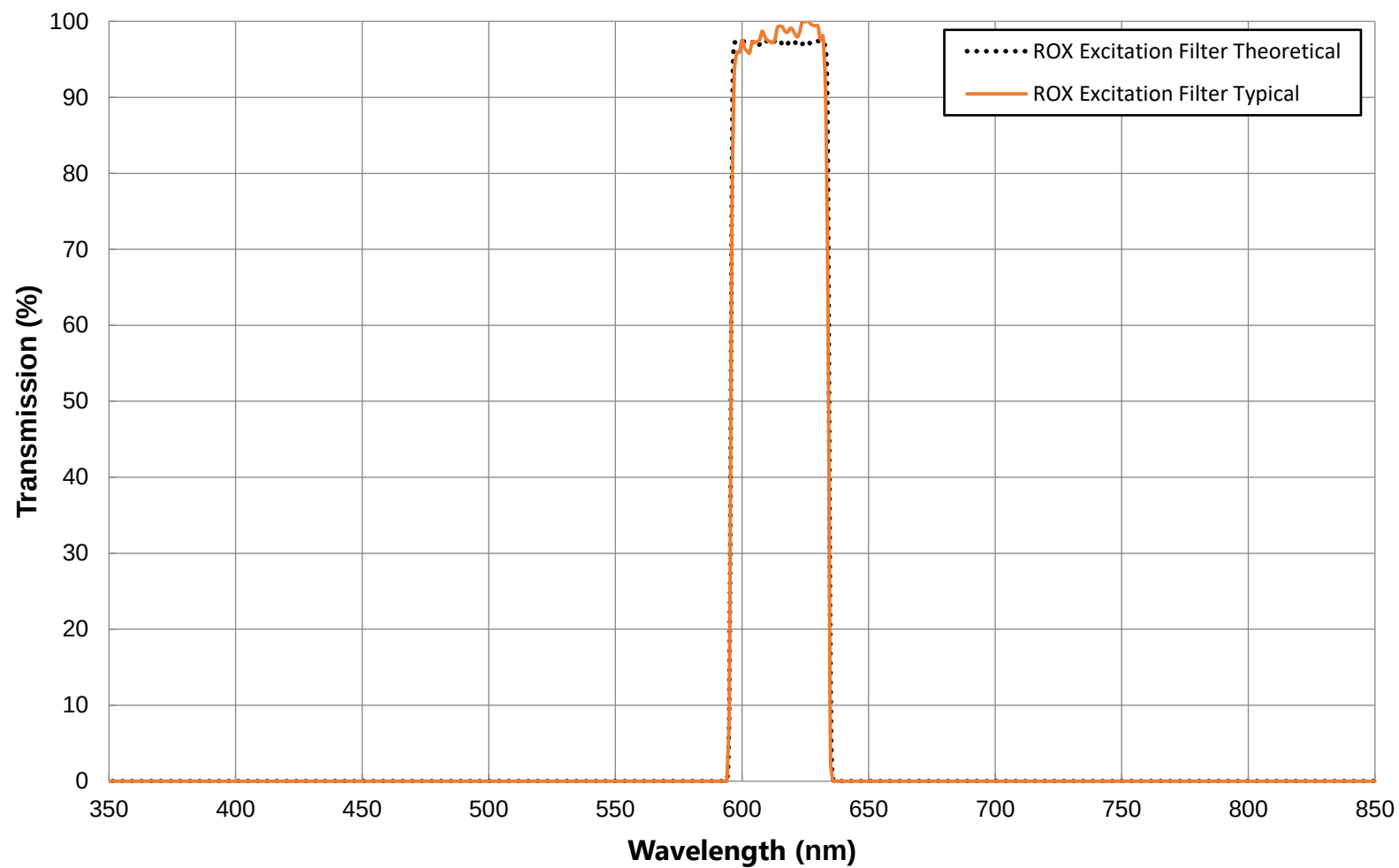
615nm CWL, OD8 High Blocking Bandpass Filter FOR REFERENCE ONLY
