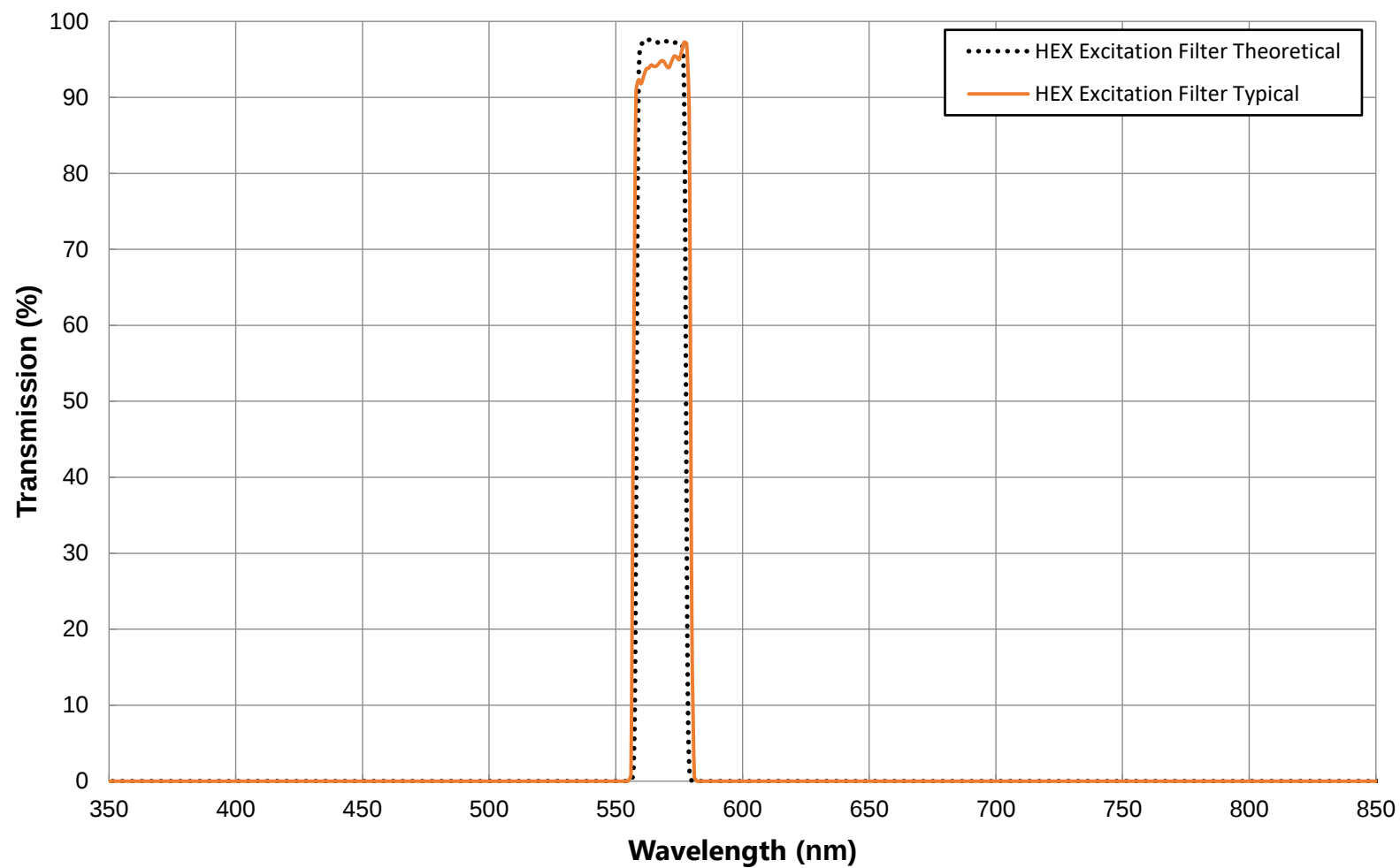
568nm CWL, OD8 High Blocking Bandpass Filter FOR REFERENCE ONLY
