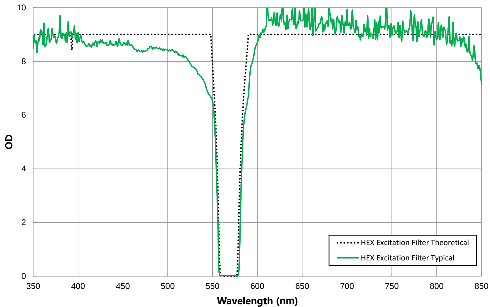
568nm CWL, OD8 High Blocking Bandpass Filter FOR REFERENCE ONLY
