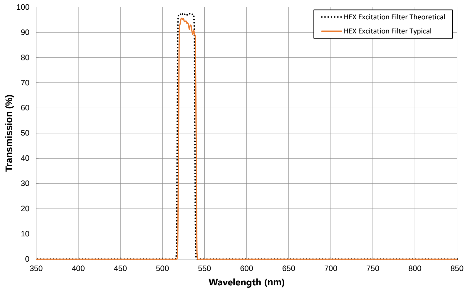
528nm CWL, OD8 High Blocking Bandpass Filter FOR REFERENCE ONLY
