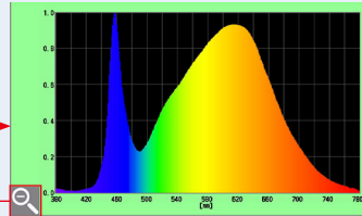
Spectrum Distribution Graph Enlarged Display
