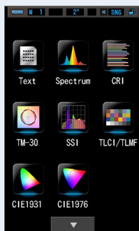
Display Mode Selection Screen Page 1
