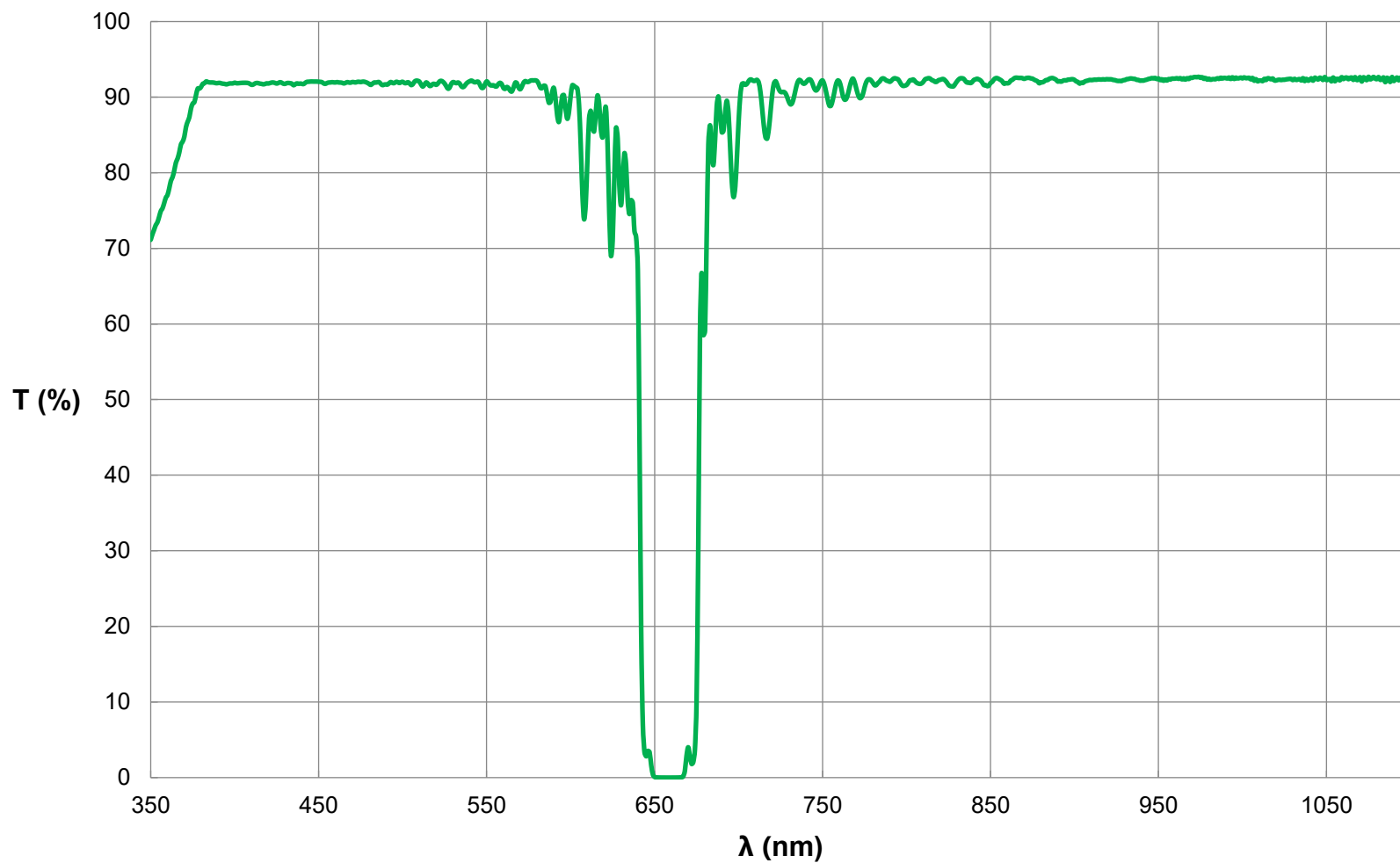
Everix Ultra-Thin OD 4 Notch Filter, 658nm, 12.5mm Diameter FOR REFERENCE ONLY
