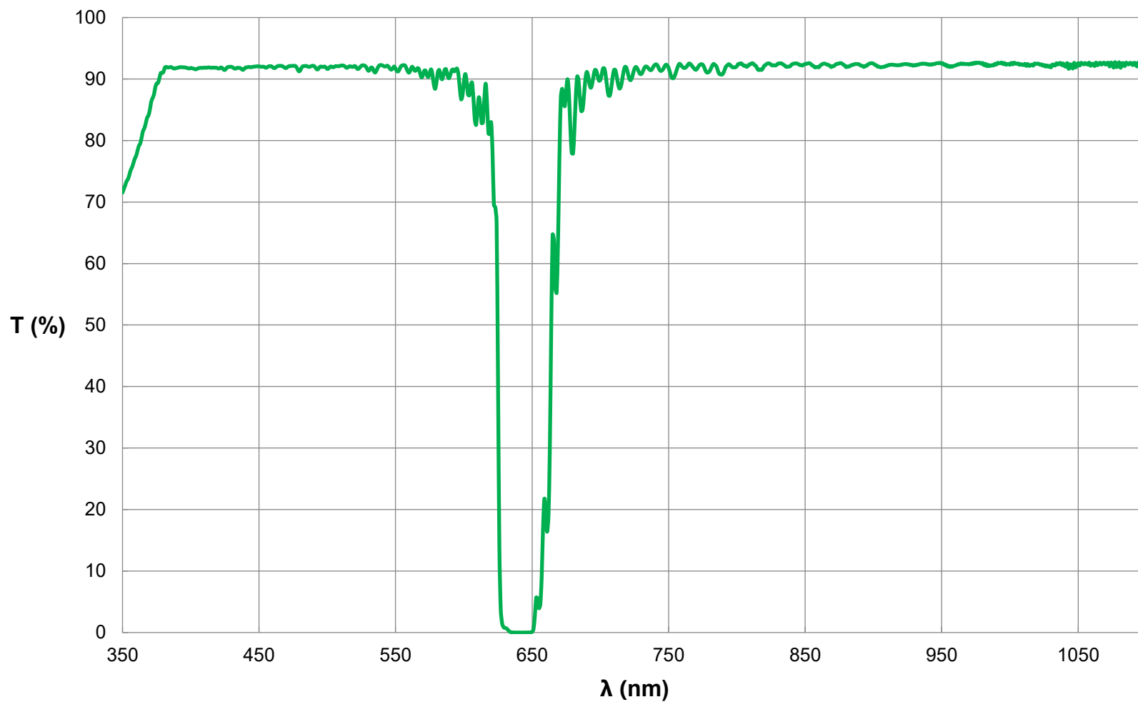
Everix Ultra-Thin OD 4 Notch Filter, 642nm, 12.5mm Diameter FOR REFERENCE ONLY
