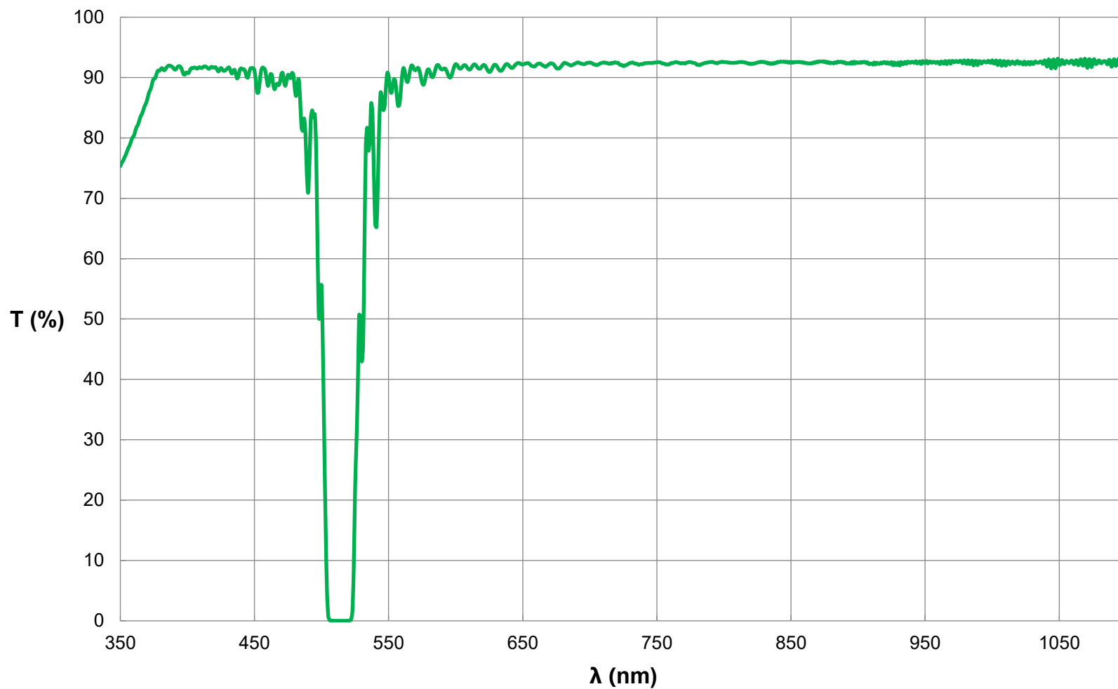
Everix Ultra-Thin OD 4 Notch Filter, 514nm, 12.5mm Diameter FOR REFERENCE ONLY
