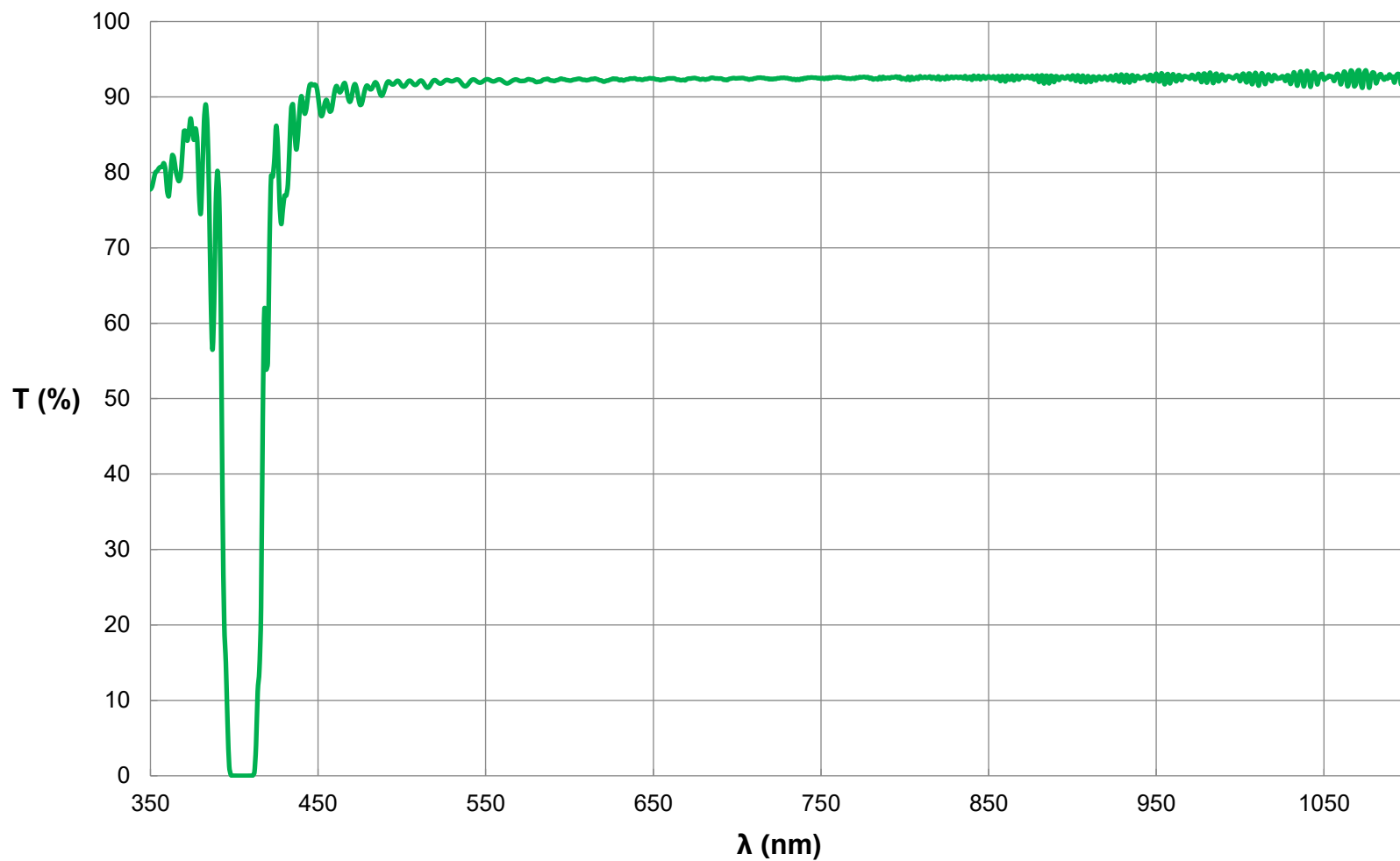
Everix Ultra-Thin OD 4 Notch Filter, 405nm, 12.5mm Diameter FOR REFERENCE ONLY
