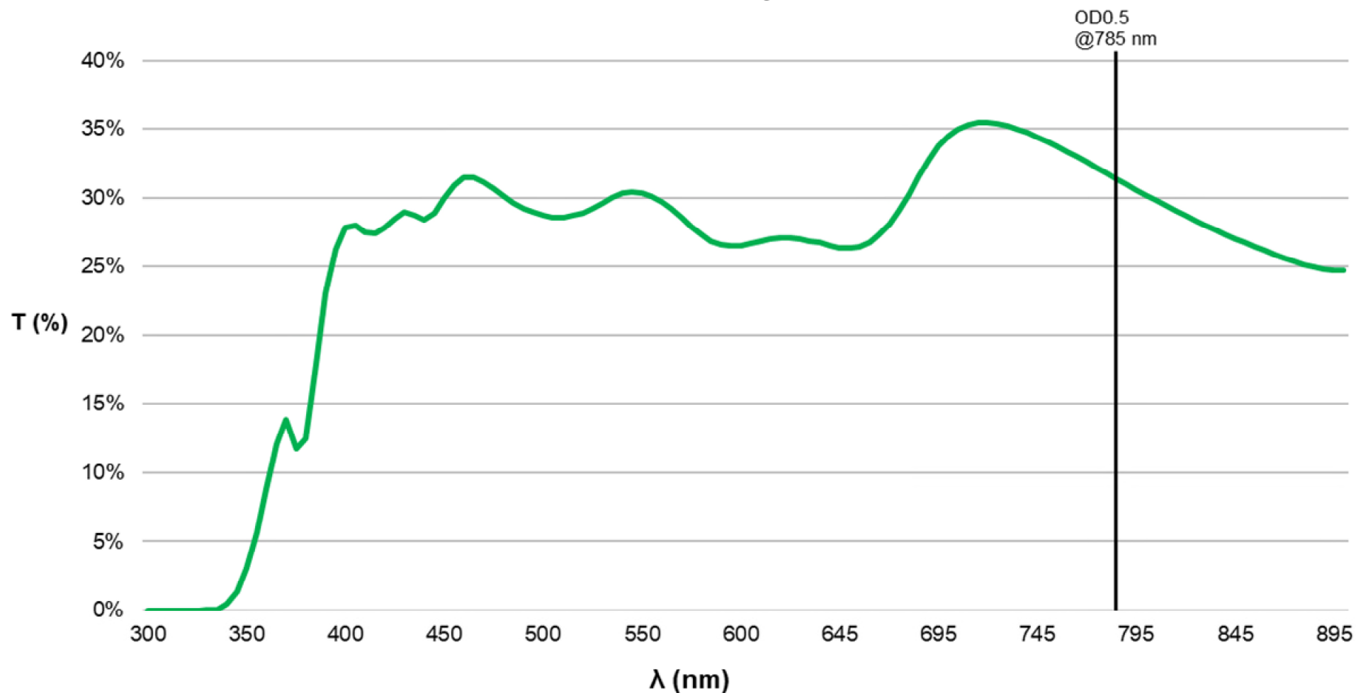
SCHOTT NG5 785 nm 50 Sq., 0.5 OD ND Filter REFERENCE Only
