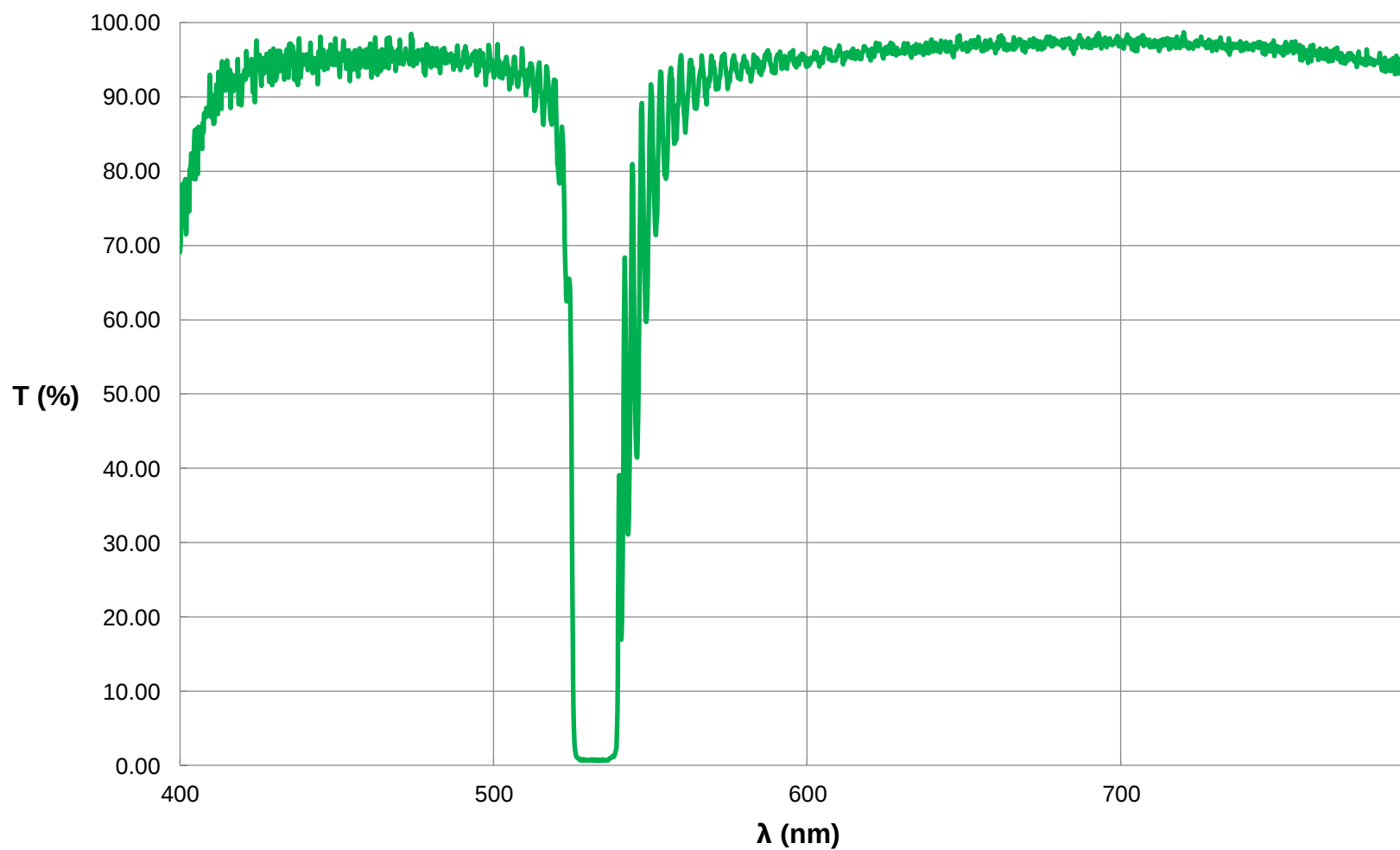
532nm META ® holoOPTIX ® STRATA Notch Filter FOR REFERENCE ONLY
